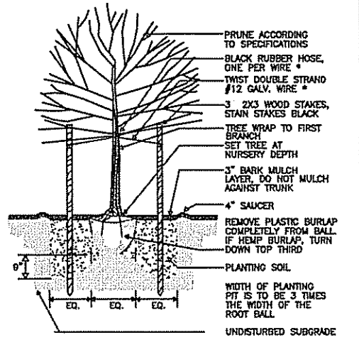
Tree Planting Detail TO BE REMOVED WITHIN ONE YEAR NOT TO SCALE
