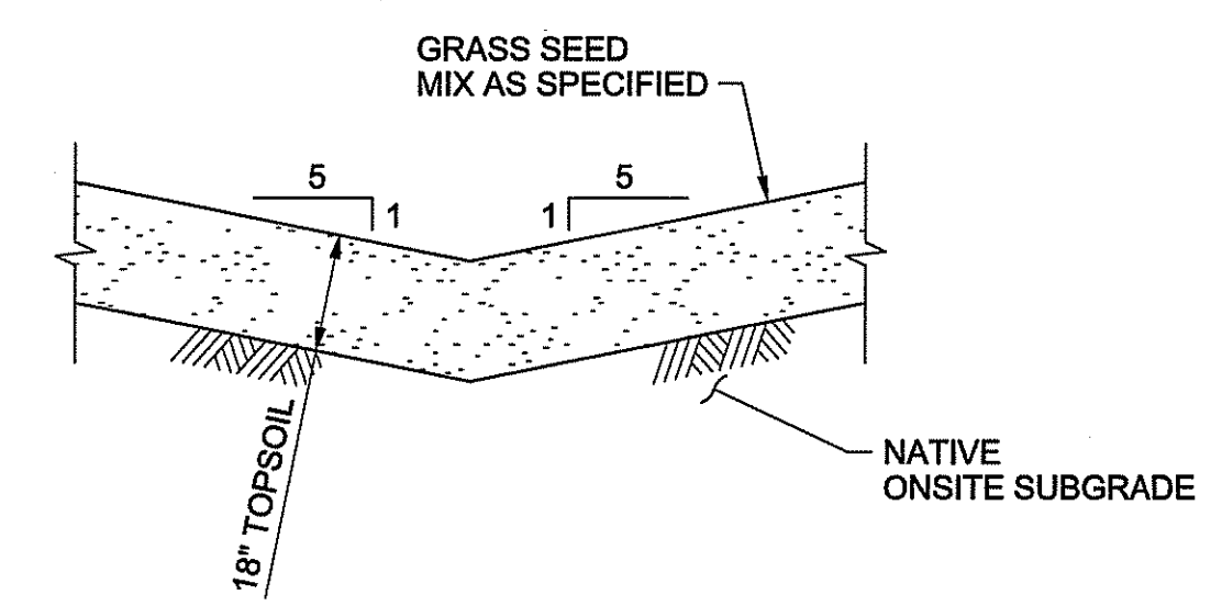
SECTION A-A 3/8"=1'-0"
