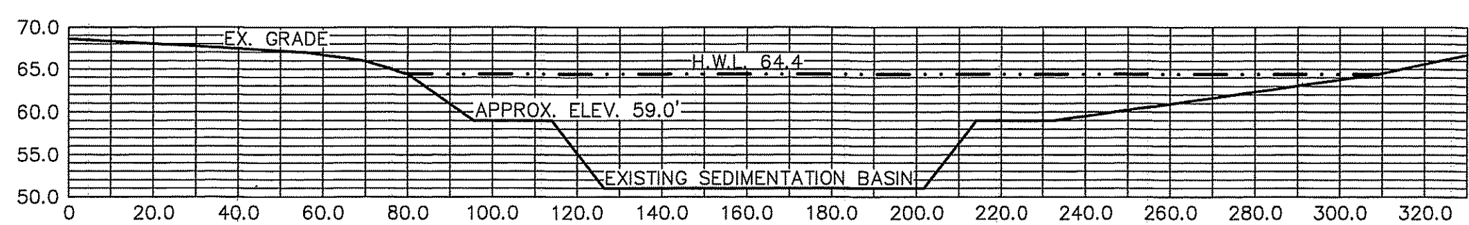
CROSS SECTION A-A SCALE: HORZ. 1"=30' VERT. 1"=15'
